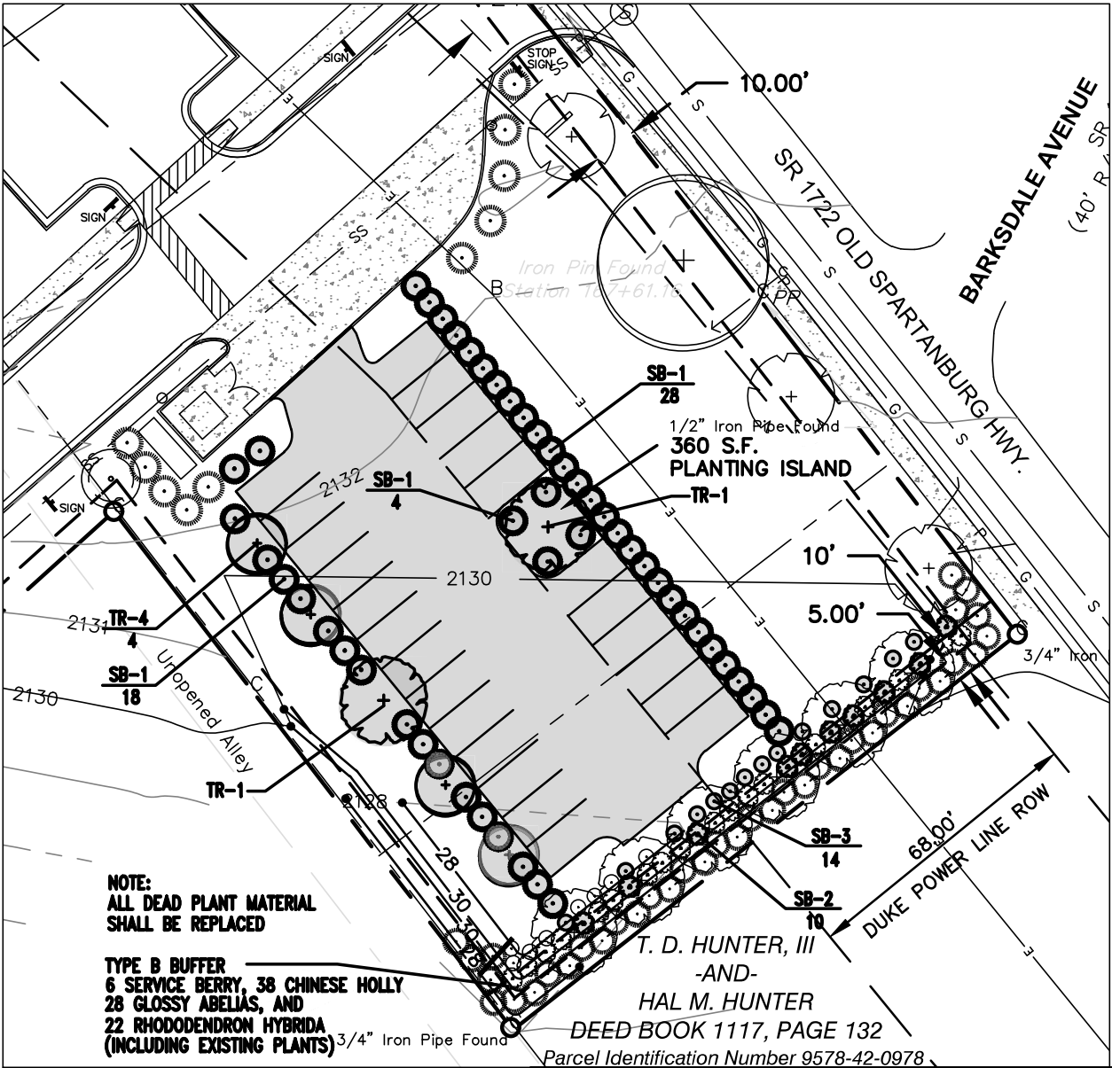
PROPOSED LANDSCAPE PLAN
