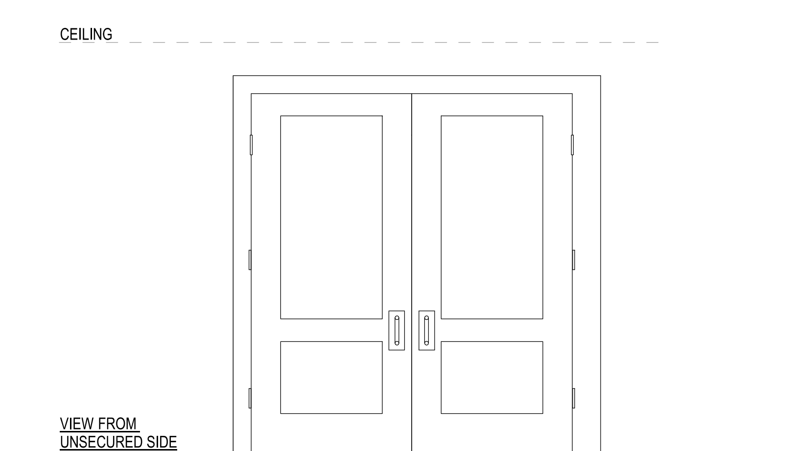
C1 SECURITY DOOR W/ AUDIBLE ALARM (WIRED) NO SCALE
